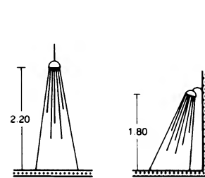
⑦ Clear height of shower heads
